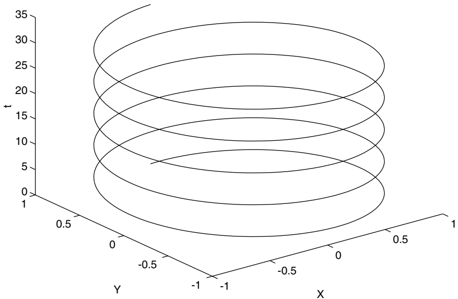
Figure 6.19 Spiral curve specified by (X, Y, Z) = [\cos(t), \sin(t), t] for t = [1, 10\pi] .
