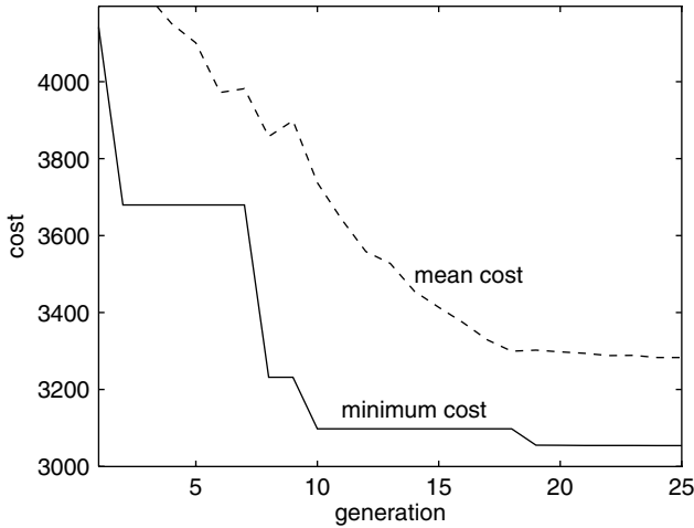
Figure 6.5 Convergence graph for the emergency response unit problem from Chapter 4 when a Gray code is used.
