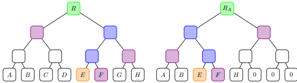
Fig. 3: A user zero-knowledge-proves two Merkle branches: one proving that their coin ID is somewhere in the coin ID tree, and another proving that that same coin ID is somewhere in the tree representing the user’s provided association set (represented by its root R_A ).
